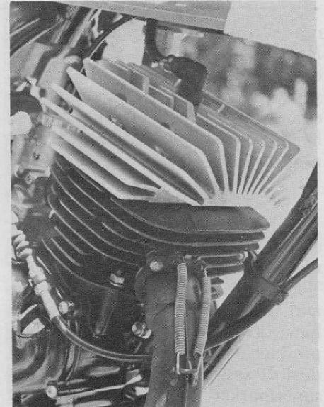
Least expensive was the DG head, a one-piece extrusion. Its high cranking pressure could negate any money saved by eating a piston.
