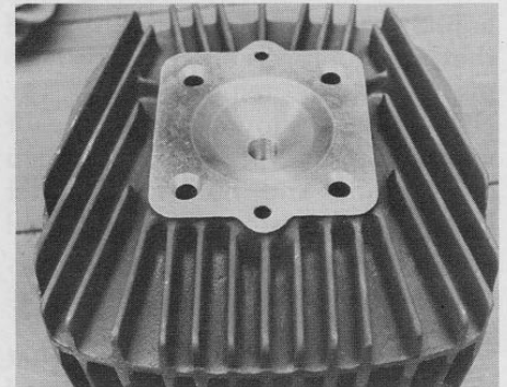
The Webco was the only head to sport underfinning.
